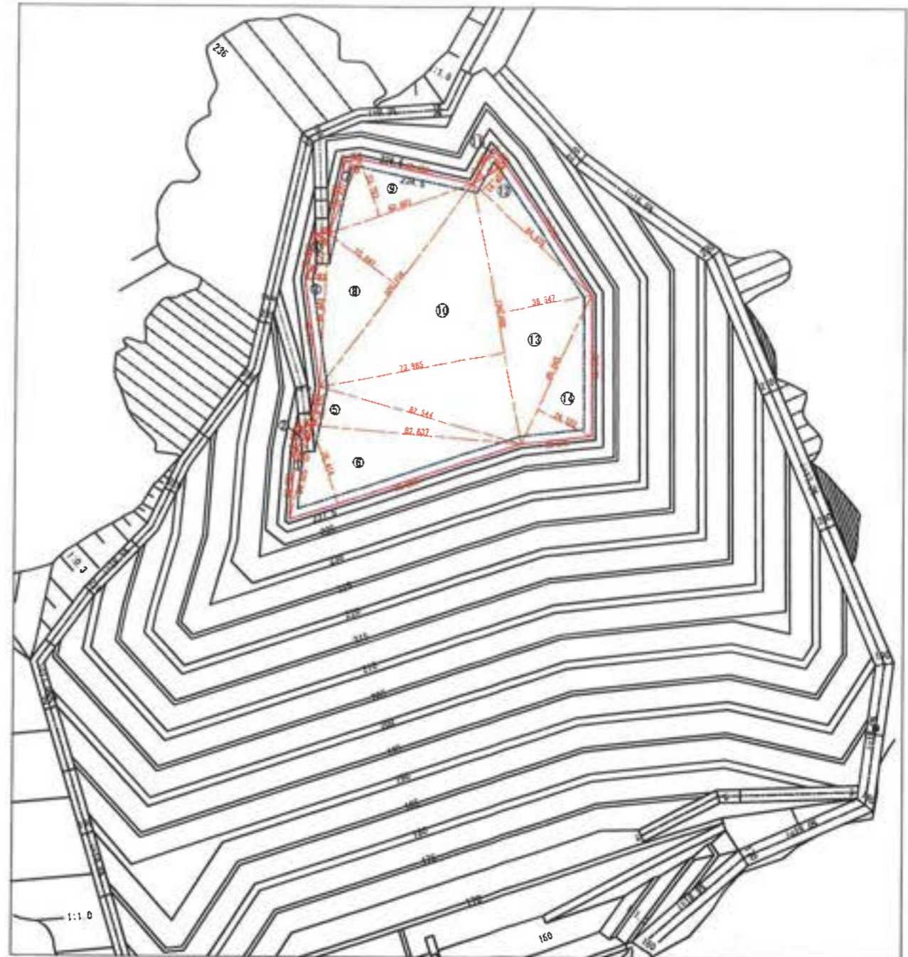
EL236.5
